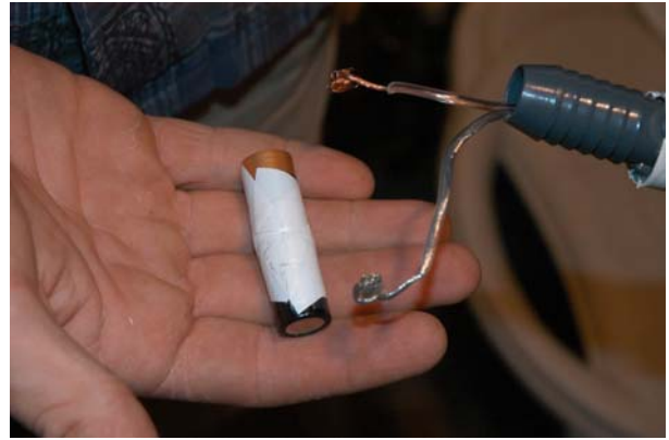
Fig. 6 Note that copper is positive (nipple end). Silver is negative (flat end)
